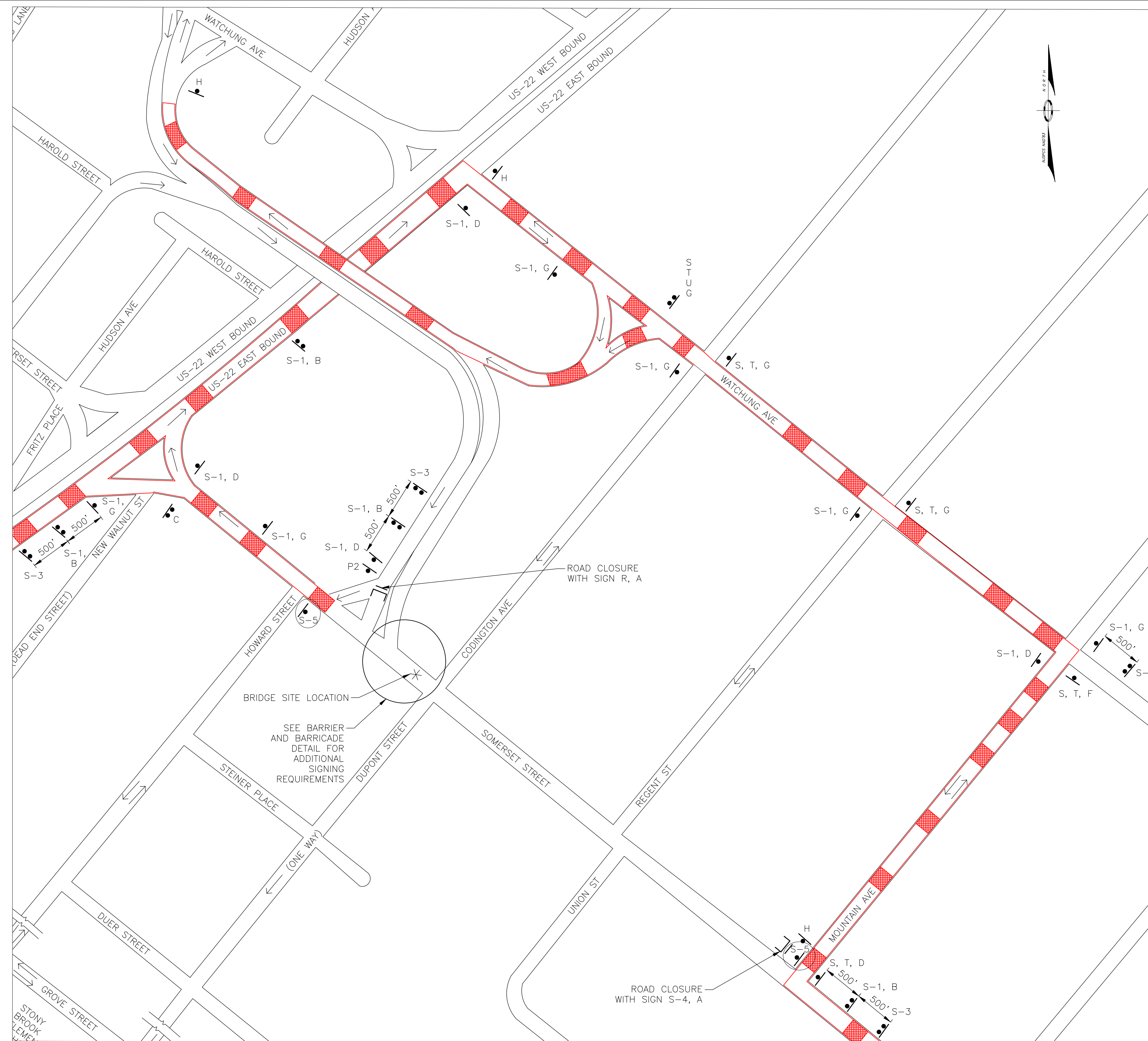
TRAFFIC DETOUR PLAN NOT TO SCALE
